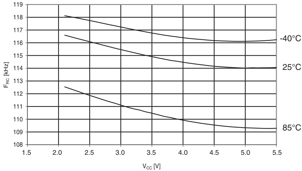
Figure 30-282. ATmega644PA: Watchdog oscillator orequency vs. V_{CC}
